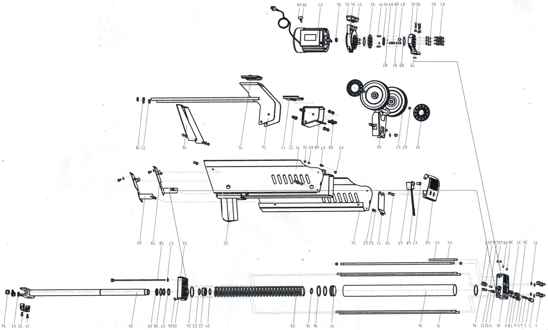
Log splitter 71
