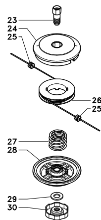
"FLASH" 31 (23+30)
