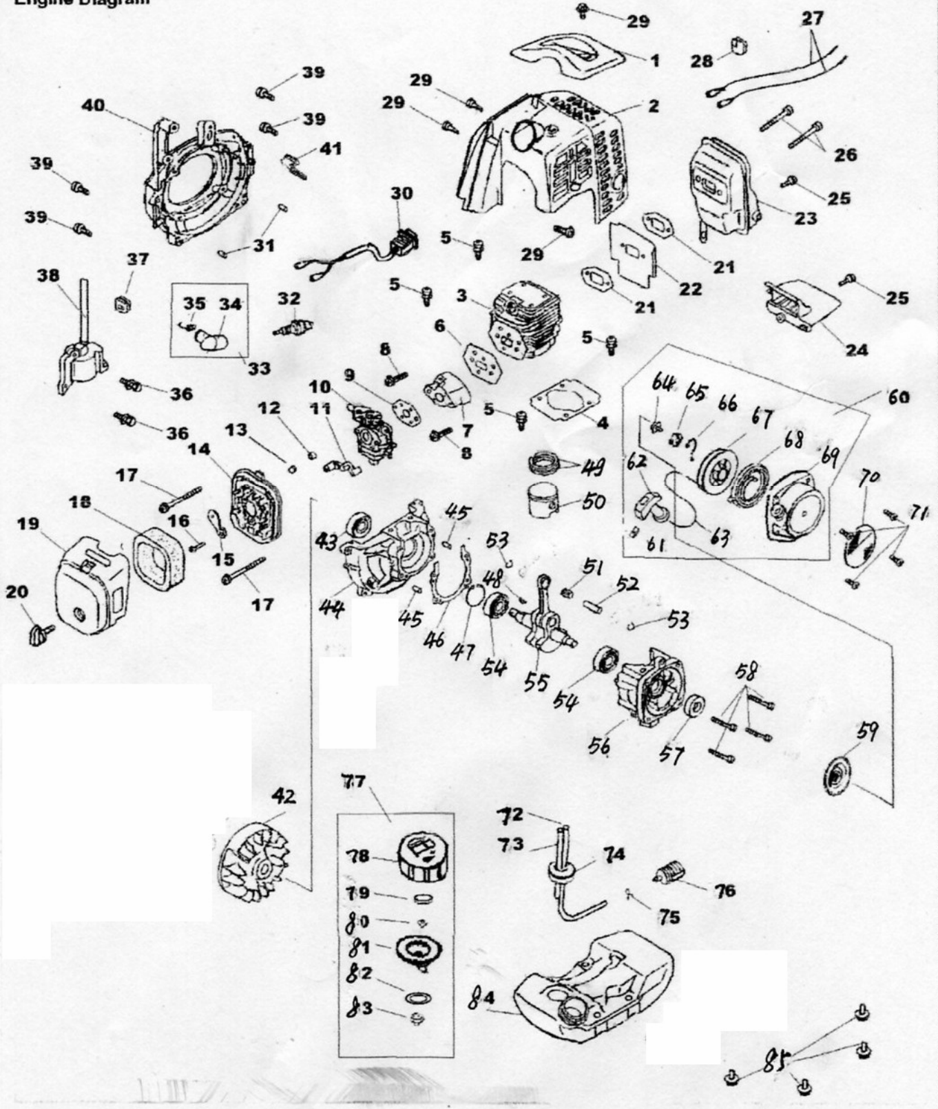
Engine Diagram
